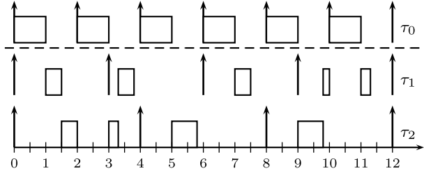
Fig. 3 Illustration that Test 4 is sufficient but not exact. The original task set, \tau_0 = (1, 2) , \tau_1 = (0.5, 3) , \tau_2 = (0.8, 4) , is schedulable while task set \tau_0 = (1, 2) , \tau'_1 = (1.1, 3) is not, where C'_1 = T_1 U(\{\tau_1, \tau_2\})
