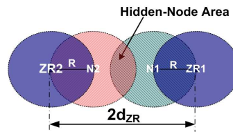
Fig. 13. Hidden-Node Area
