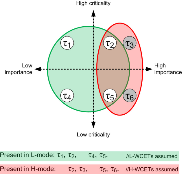
Fig. 1: A Venn diagram illustrating the different types of tasks in our task model, the modes that they can be part of and the WCET estimates used for schedulability-testing purposes.
